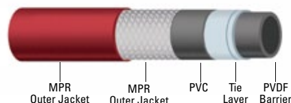
FUEL LINE TUBING CONSTRUCTION
